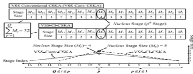
Fig. 4. Sizes of the stages in the case of VSS for the proposed and conventional 32-bit CSKA
