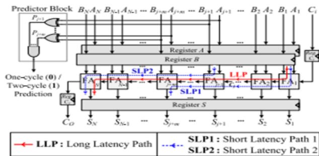
Fig. 5. Generic structure of variable latency adders based on RCA.
