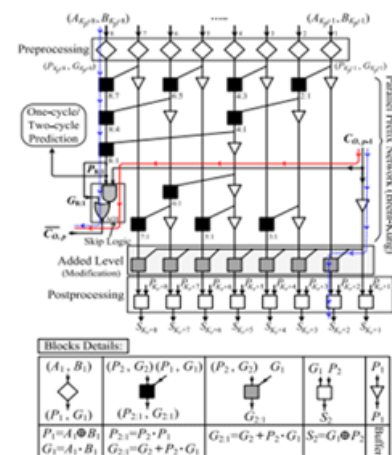
Fig. 7. Internal structure of the pth stage of the proposed hybrid variable latency CSKA. M_p is equal to 8 and K_p = \sum_{r=1}^{j-1} M_r .
