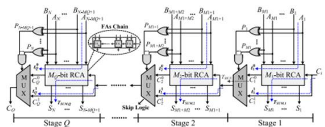
Fig. 1. Conventional structure of the CSKA [19].
