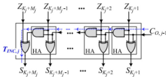
Fig. 3. Internal structure of the j th incrementation block, K_j = \sum_{r=1}^{j-1} M_r ( j = 2, \dots, Q ).
