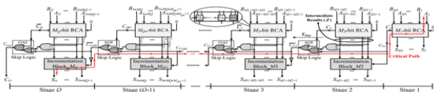
Fig. 2. Proposed CI-CSKA structure
