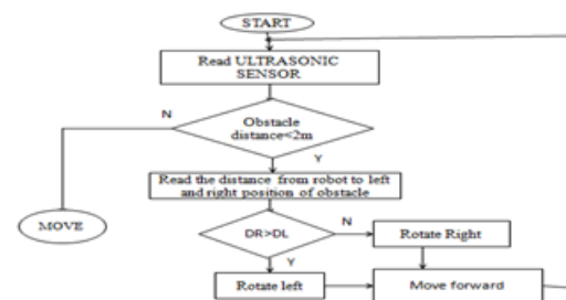
Fig-8: Obstacle avoidance process
