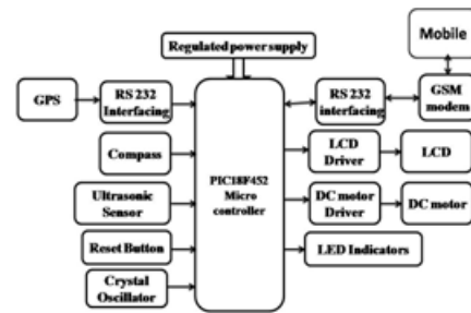
Fig-1: Block diagram of Autonomous robot
