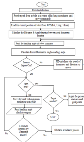
Fig-7: Navigation system
