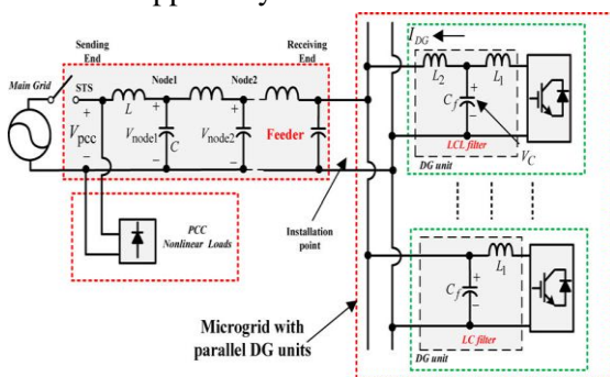
Fig.2. Simplified one-line diagram of a single-phase microgrid.
