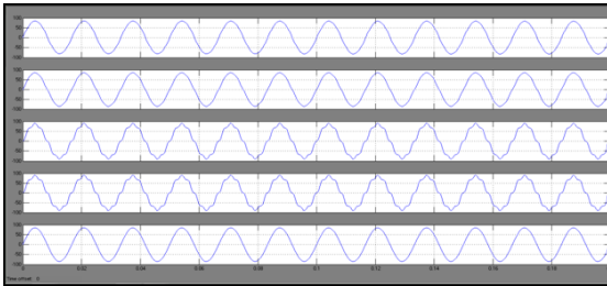
Fig 10 Harmonic voltage amplification during a single DG unit grid connected operation (with virtual nonlinear capacitor and resistor based active damping by using fuzzy logic) (a) PCC voltage (b) node 1 voltage (c) node 3 voltage (d) node 5 voltage (e) DG unit filter capacitor voltage.
