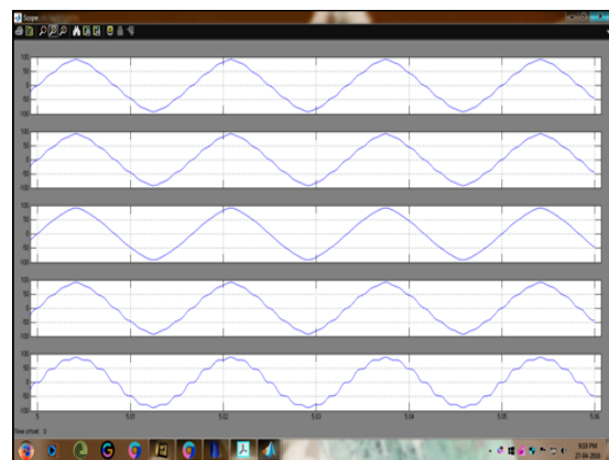
Fig 7 Harmonic voltage amplification during a single DG unit islanding operation (with virtual nonlinear capacitor and resistor based active damping) (a) PCC voltage (b) node 1 voltage (c) node 3 voltage (d) node 5 voltage (e) DG unit filter capacitor voltage.
