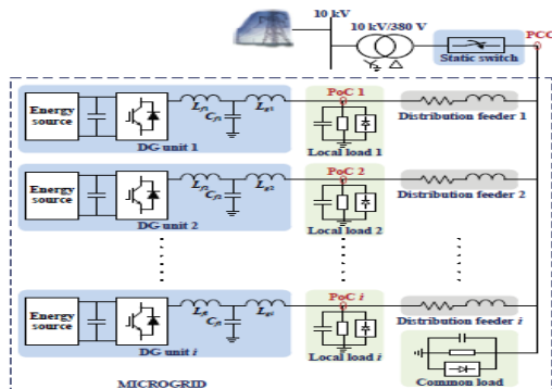
Fig.1. A sample low-voltage microgrid dominated with multiple inverter interfaced DG units.
