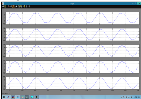
Fig 4 Harmonic voltage amplification during a single DG unit grid connected operation (without damping) (a) PCC voltage (b) node 1 voltage (c) node 3 voltage (d) node 5 voltage (e) DG unit filter capacitor voltage.
