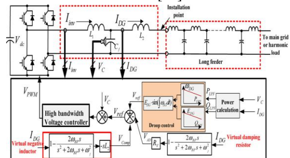
Fig. 3. Mitigation of distribution feeder harmonic propagation using virtual resistor and virtual negative inductor.
