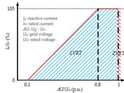
Fig. 6. Reactive current injection requirements under low-voltage ride-through/zero-voltage ride-through (LVRT/ZVRT) operations.
