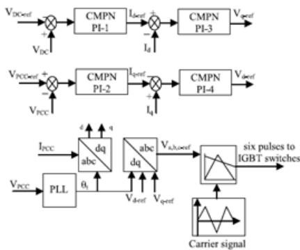
Fig. 4. Control block diagram of the grid-side inverter.
