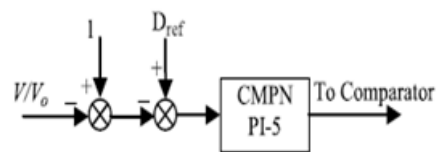
Fig. 3. Control of the DC-DC converter.
