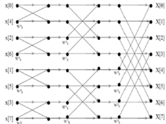
Fig.3. signal flow graph of 8 point DIT radix-2 FFT
