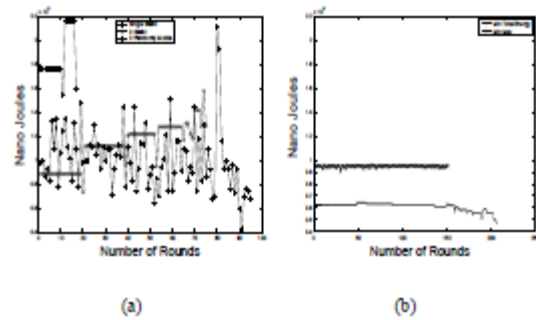
Fig. 5. Energy Spent in Each Round
