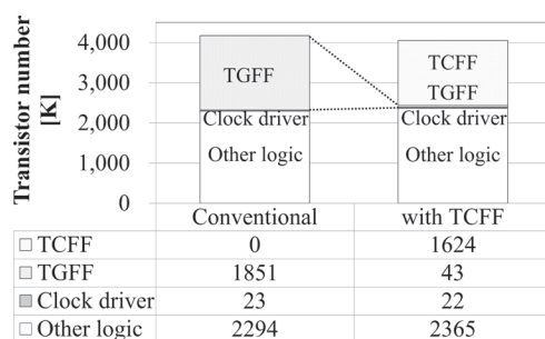
Fig. 24. Transistor count of random logic area with and without TCFF.
