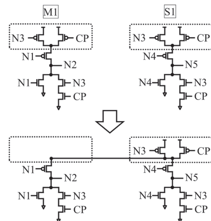
Fig. 9. Transistor merging in PMOS side.
