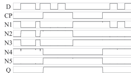
Fig. 14. Waveform on SPICE simulation.
