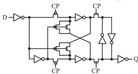
Fig. 5. Adaptive-coupling flip-flop (ACFF).
