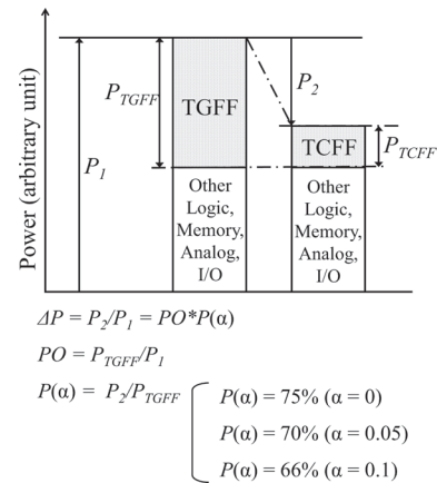
Fig. 25. Power reduction estimation in a chip.
