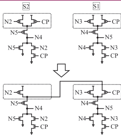
Fig. 11. Further transistor merging in PMOS side.
