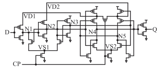
Fig. 13. Transistor level schematic of topologically-compressed flip-flop (TCFF).
