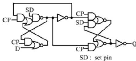
Fig. 17. TCFF with set type.
