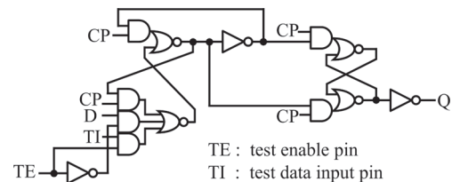
Fig. 15. TCFF with scan type.
