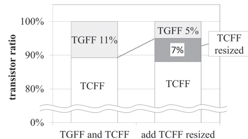
Fig. 26. Frequency dependence of replacement from TGFF to TCFF and the resized TCFF.
