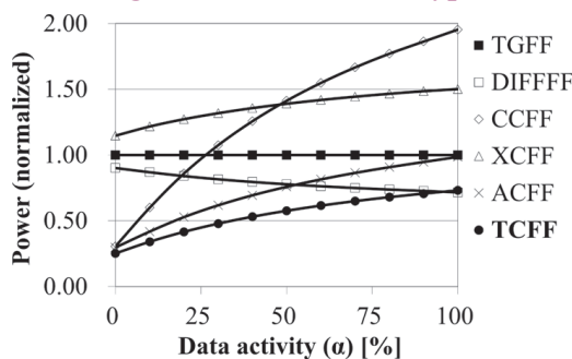
Fig. 17. TCFF with set type.
