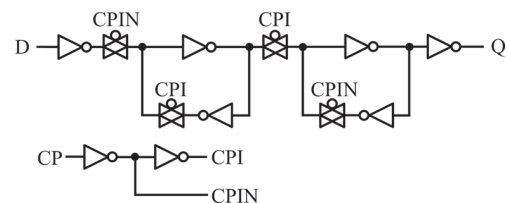
Fig.1. Conventional transmission-gate flip-flop (TGFF).
