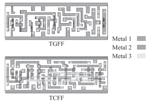
Fig. 22. The cell layout with scan.
