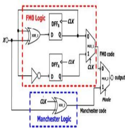
Hardware architecture
