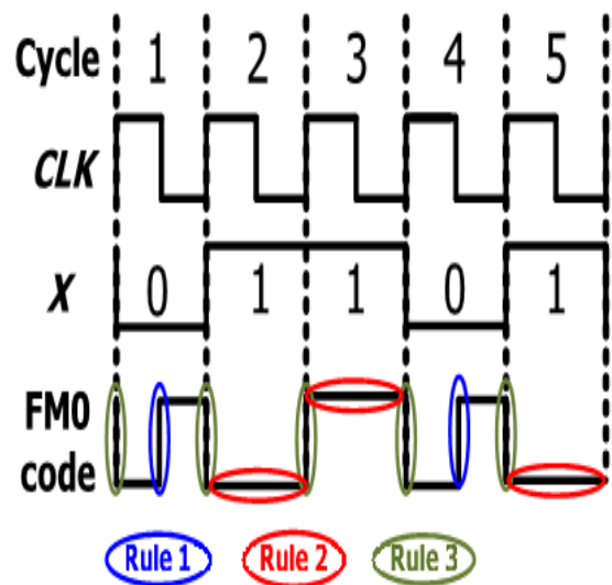
Illustration of FM0 coding example.
