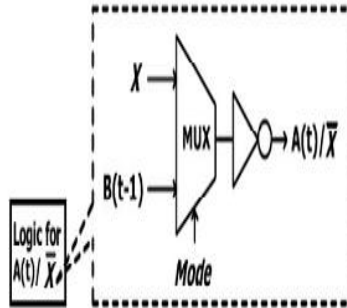
FM0 encoding with area compact retiming.
