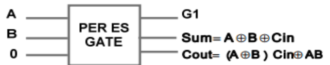
Figure4. Peres gate as half adder
