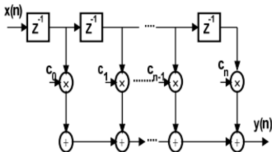
Figure.1 Direct form FIR Filter structure
