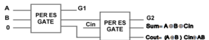
Figure.5 Peres gate as full adder
