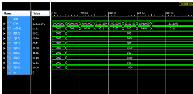
Figure15: Simulation results of Reversible 8-Tap FIR using Carry Look Ahead adder and Wallace Treemultiplier
