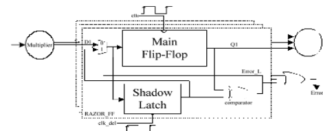
Fig. 6. Razor flip flops
