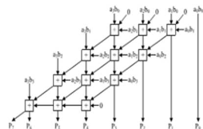
Fig 2. 4 \times 4 normal AM.
