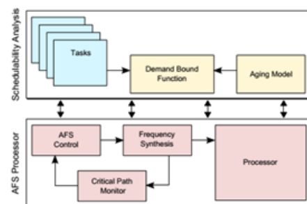
Fig. 1. Schematic view of an AFS processor
