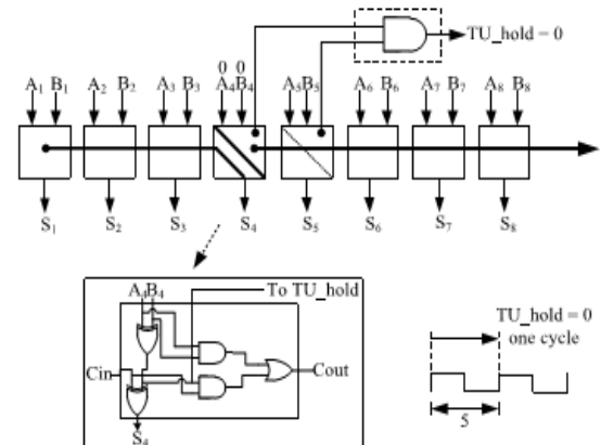
Fig. 4. 8-bit RCA with a hold logic circuit.
