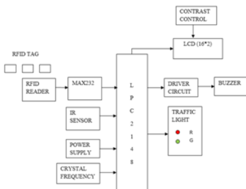
Figure. 3.1 Architecture diagram
