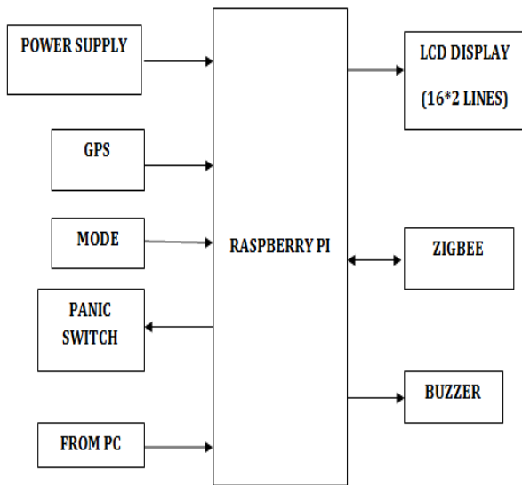
Block Diagram of the Transmitter
