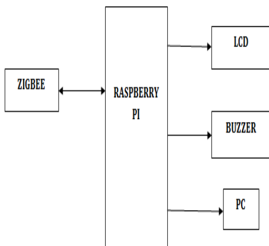
Block Diagram of the Receiver
