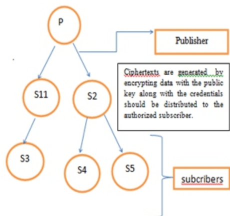
Fig: Data sharing between publisher and subscriber using identity based encryption
