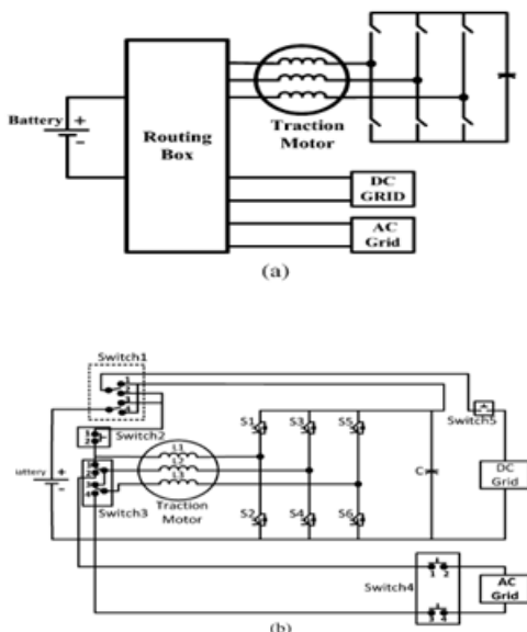
Fig. 1. Converter with switches capable of interfacing with both ac and dc grid (a) combined and (b) details
