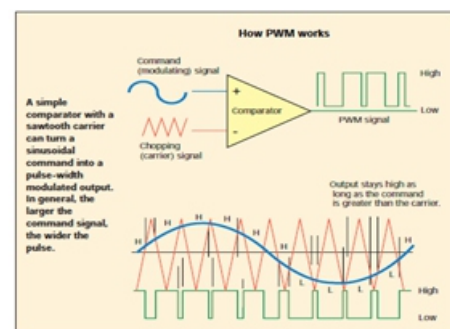
Fig.2. PWM Strategy
