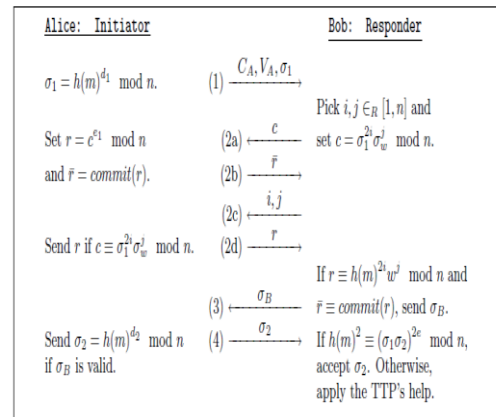
Figure 1: Signature Exchange Protocol.
