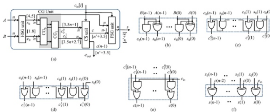
Fig. 3.(a) Proposed CS adder design, where n is the input operand bit-width, and [ ] represents delay (in the unit of inverter delay), n = \max(t, 3.5n + 2.7) . (b) Gate-level design of the HSG. (c) Gate-level optimized design of (CG0) for input-carry = 0. (d) Gate-level optimized design of (CG1) for input-carry = 1. (e) Gate-level design of the CS unit. (f) Gate-level design of the final-sum generation (FSG) unit.
