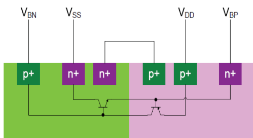
Figure 3: Leakage path in forward body biasing
