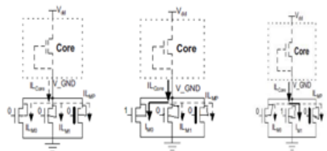
Figure: 2 Proposed architecture: (a) Snore mode (b) Dream mode (c) Sleep mode
