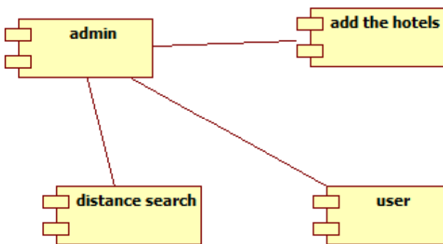
Figure.11. Component diagram
