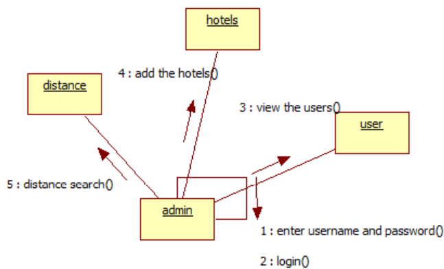
Figure.8. Collaboration Diagram.
