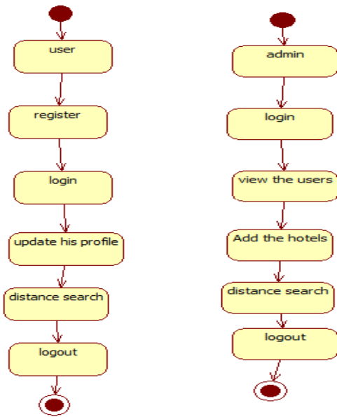
Figure.10. Admin & User Activity diagrams
