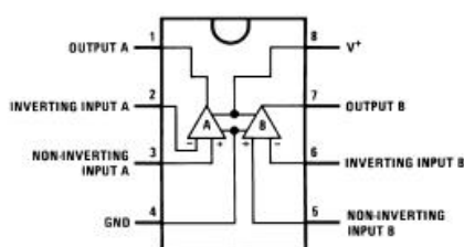
Fig.4 Image of LM358 comparator.
