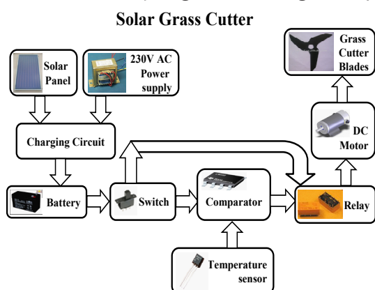
Figure- 2. Image of Block Diagram of Proposed model
