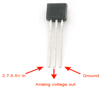
Fig.7. Temperature sensor
