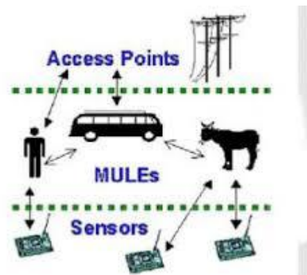
Figure 3: The three tiers of the MULE architecture
