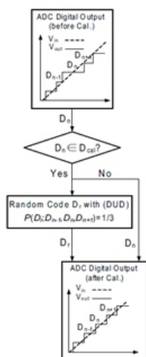
Fig. 4. Code-randomized calibration algorithm.
