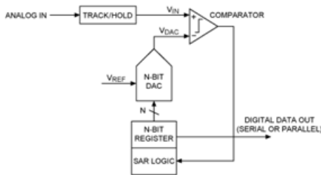
Fig. 1. Block diagram of the ADC architecture.
