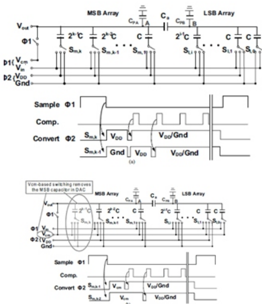
Fig. 2. Single-ended n-bit and (n - 1)-bit split capacitive DAC arrays with their switching timing diagrams (n = k + i). (a) Conventional switching. (b) Vcm-based switching.
