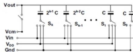
Fig. 3. k-bit binary-weighted DAC.
