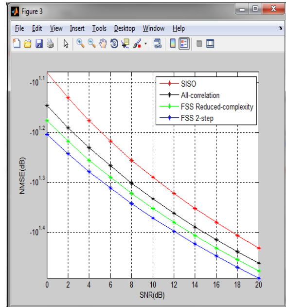
Fig. 2. Prediction performance of a high correlation scenario ( \alpha = 0.9, \beta = 0.9), M = 4, N = 2, Doppler frequency is 70 Hz.
