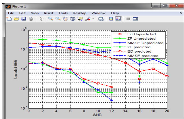
Figure 1 Performance of pre coding with predicted channel coefficient of a high correlation scenario ( \alpha =
