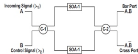
(a) Semiconductor Optical Amplifier Based MZI
