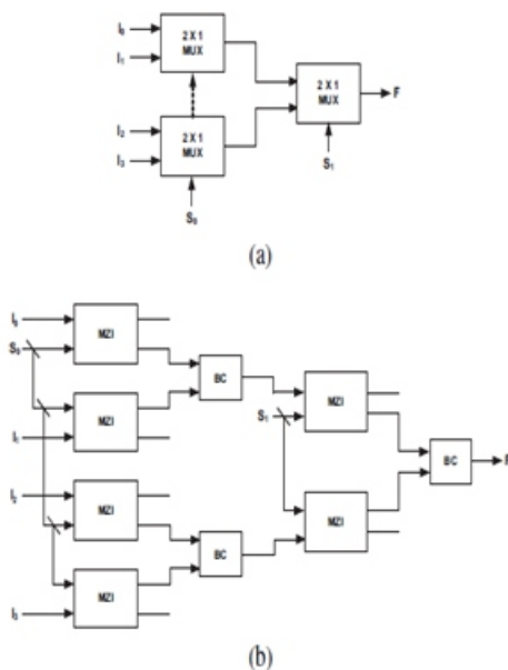
Fig. 5. A 4-to-1 MUX (a) schematic diagram, (b) all-optical implementation
