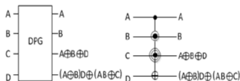
Fig. 5a. Double Peres gate Fig.5b. Graphical representation.
