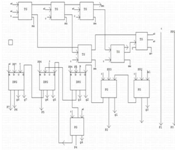
Fig. 11. Complete Reversible circuit of 4 bit square unit
