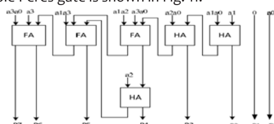
Fig.8. Summation circuitry for 4x4 square unit
