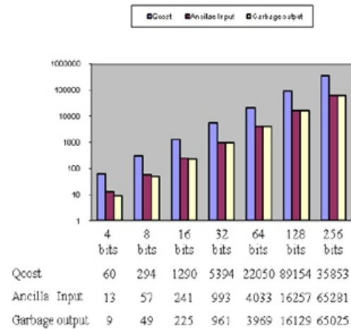
Fig. 12. Reversible circuit metrics variation for variable bit length of square
