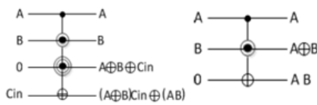
Fig. 9. DPG gate as full adder Fig. 10. Peres gate as half adder
