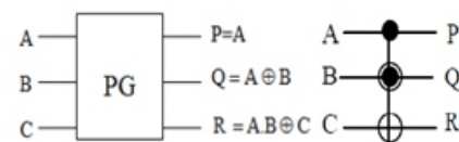
Fig. 3a. Peres gate Fig.3b. Graphical representation C.Toffoli Gate (TG)
