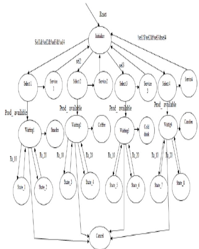
Figure 4: Finite State Machine Diagram of Vending Machine
