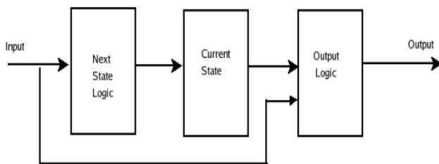
Figure 1: MEALY Machine Model
