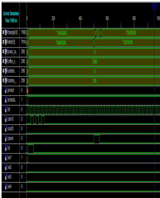
Figure 6: Simulated results of 4 candies vending machine.
