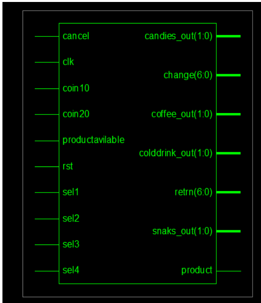
Figure 5: RTL schematic of 4 candies vending machine.
