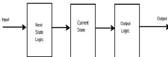
Figure 2: MOORE Machine Model
