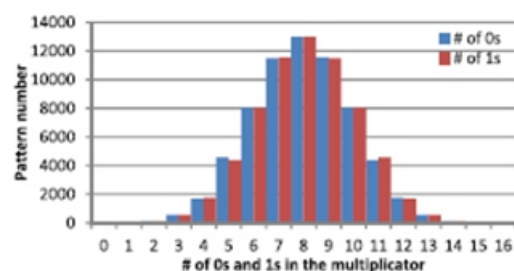
Fig: pattern number distribution based on the number of 0s and 1s in the multiplier
