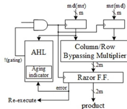
Fig: Proposed architecture (md means multiplicand; mr means multiplier).
