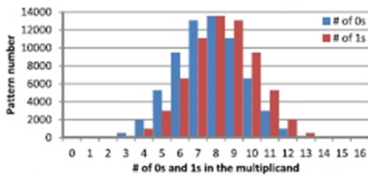
Fig: pattern number distribution based on the number of 0s and 1s in the multiplicand
