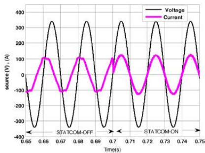
Fig. 9. Supply Voltage and Current at PCC.
