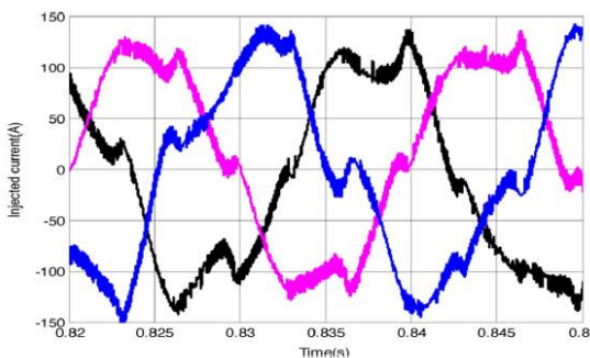
Fig. 5. Three phase injected inverter Current.
