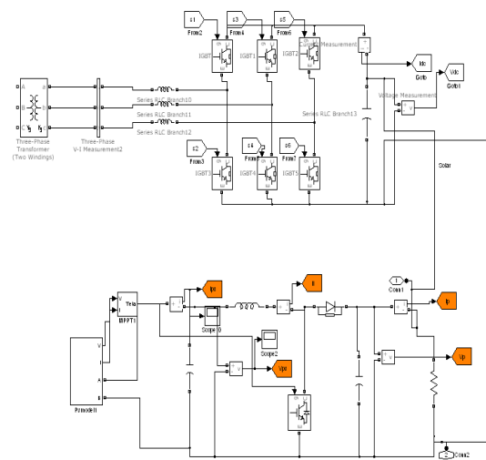
Fig 2.proposed simulation circuit PV grid connected system for power quality improvement
