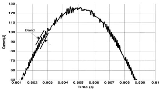
fi Fig. 4. Switching signal within a control hysteresis band.
