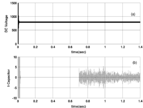
Fig. 7. (a) DC link voltage. (b) Current through Capacitor.
