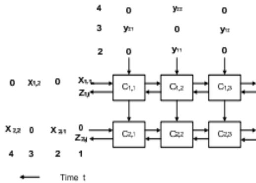
Fig. 6. Systolic array for 2 \times 2 matrix multiplication
