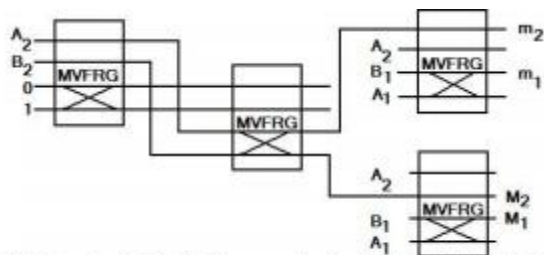
Fig. 4. Single cell of a Systolic Array using four Multiple Valued Fredkin Gates
