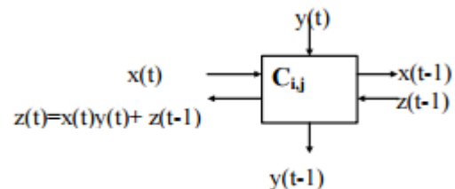
Fig. 5. Systolic array cell structure
