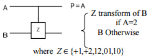
Fig. 1. Symbol of M-S gate
