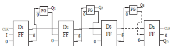
Fig.15. Edge-triggered N-bit SIPO registers using D-FF
