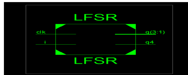
Fig 22.RTL schematic of pulse triggered reversible LFSR
