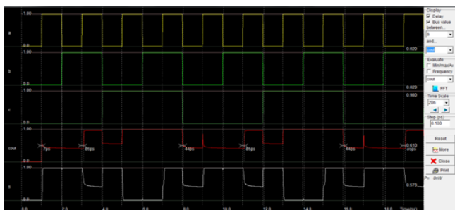
Fig 7 Layout Simulation of single gate MOSFET full adder
