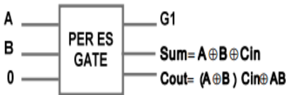
Figure. Peres gate as half adder
