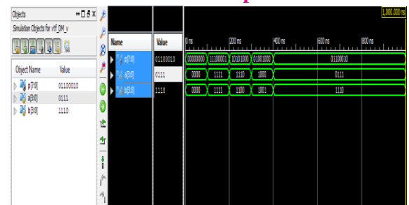
Figure13: simulation results of Reversible Dadda multiplier
