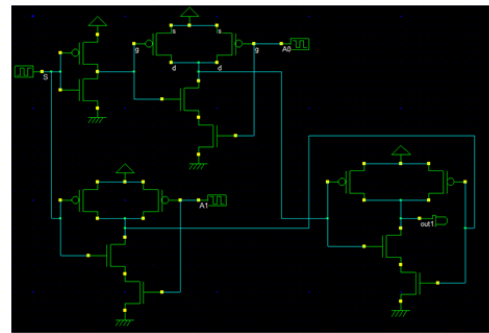
Fig.3.1 Schematic of 2 To 1 Multiplexer Using NAND Gates
