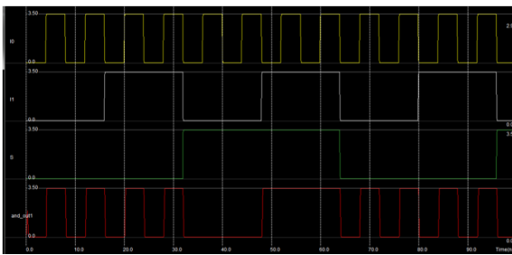
Fig.3.5 Simulation Result Of 2 To 1 Multiplexer
