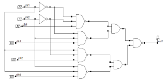
Fig2- 4:1 MUX Schematic
