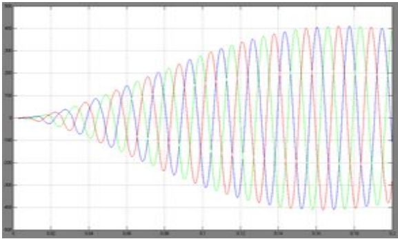
Grid voltage
