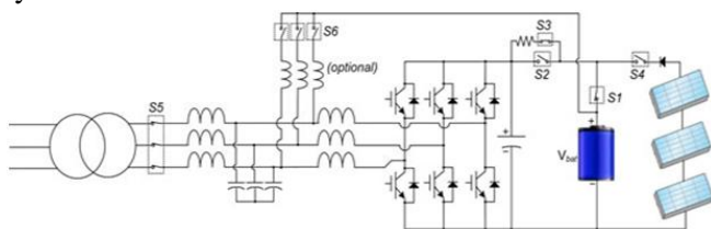
Diagrammatic representation of proposed RSC circuit
