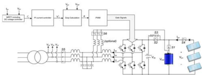
Block diagram representation of the RSC in the dc/dc operation.
