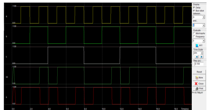
Fig 8: Simulation of Layout of 28TFull adder
