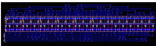
Fig 11: Layout of 12T Full adder
