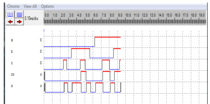
Fig 6: Timing Diagram of 28TFull adder
