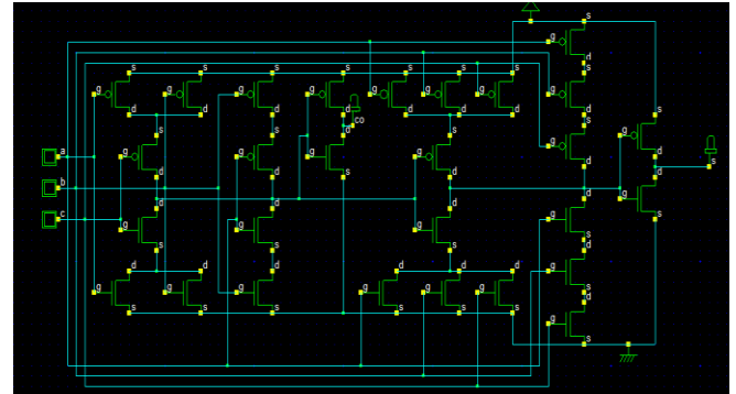
Fig 5: Schematic of 28TFull adder
