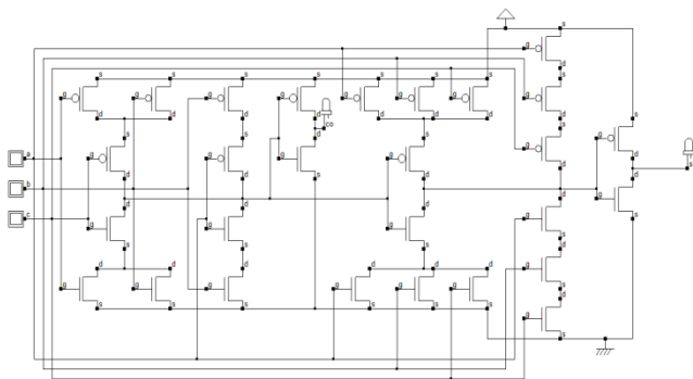
Fig. 1. Conventional 28-T CMOS 1 bit full adder
