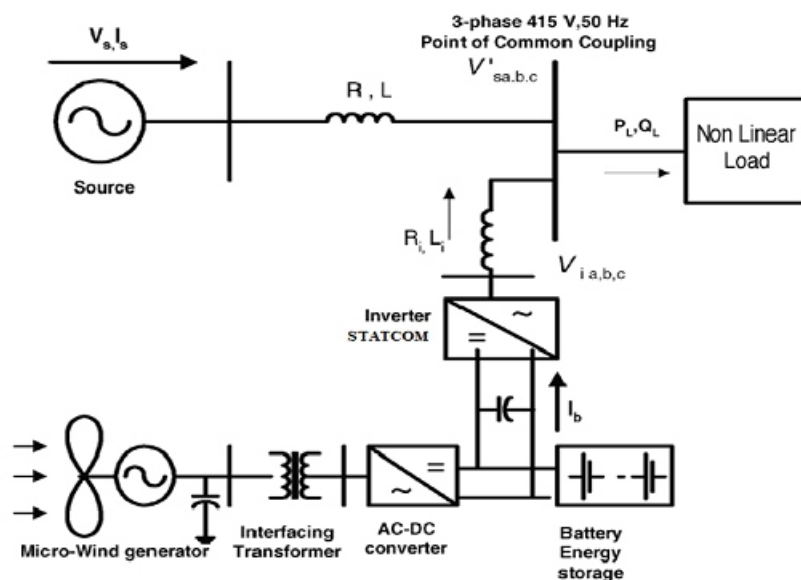
Scheme of wind generator with battery storage
