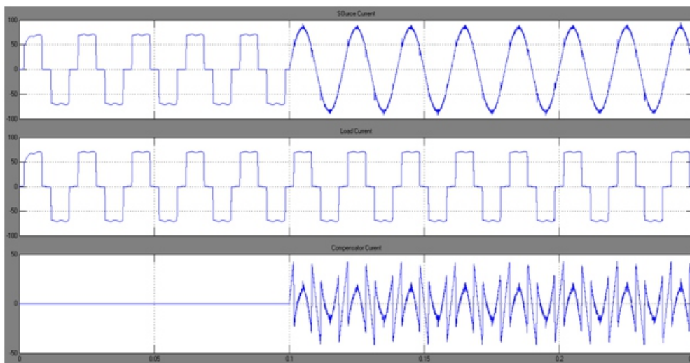
Figure 6.3: simulated wave forms of proposed system single phase source current, load current and compensator current
