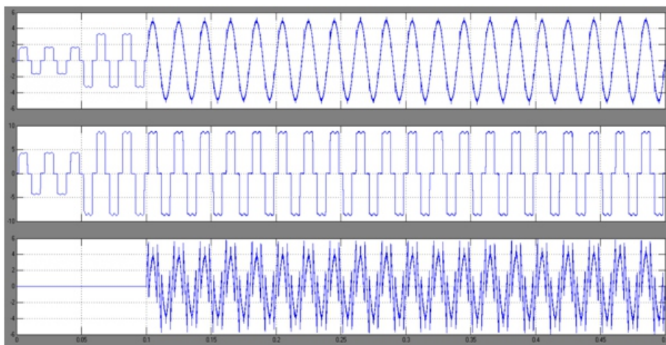
Figure 6.6: Simulated wave forms of 4-leg converter single phase source current, load current and compensator current
