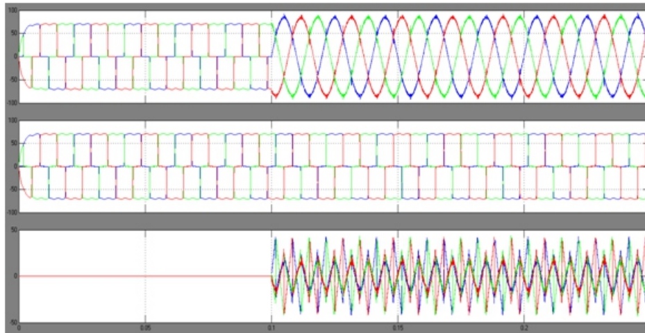
Figure 6.4: Simulated wave forms of proposed system three phase source current, load current and compensator current
