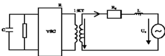
Single-phase equivalent circuit of STATCOM
