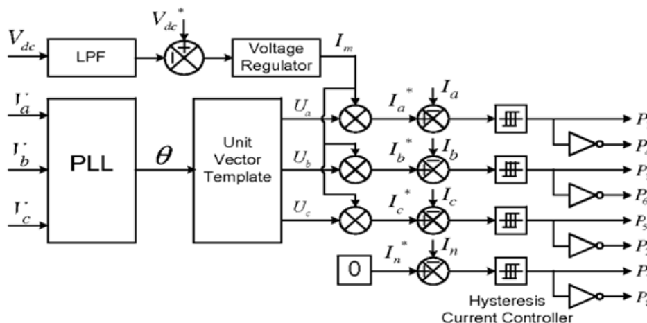
Block diagram representation of grid-interfacing inverter control.
