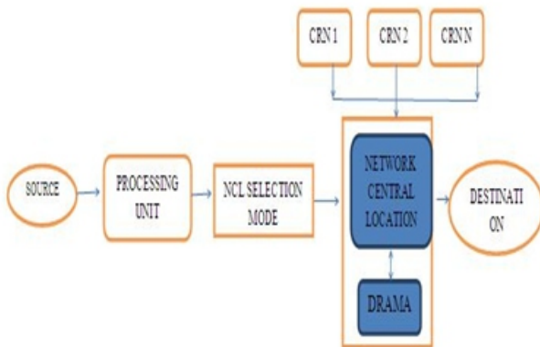
Fig 6: System architecture
