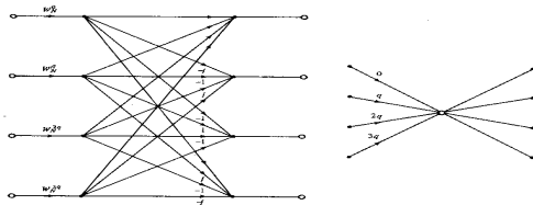
Fig4: Butterfly unit
