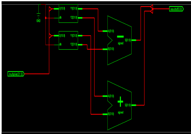
Fig8: Internal RTL Schematic
