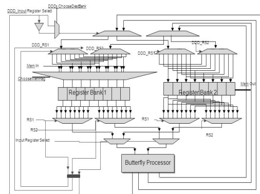
Fig3: Internal architecture of FFT The FFT processor has a modular design and comprises of 3 modules.
