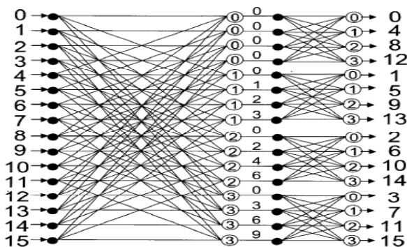
Fig.2.Signal flow graph of a radix-4 16 point FFT
