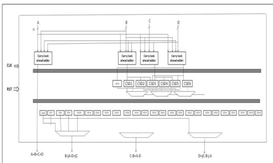
Fig5: Address generation unit
