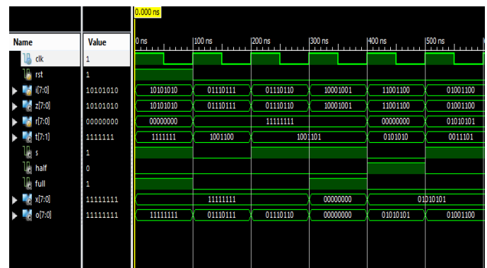
Fig.10. Scheme 2 Decoder. Decoder Scheme 3
