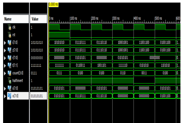
Fig.9. Scheme 1 Decoder. Decoder Scheme 2
