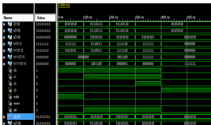
Fig.8. Scheme 3 Encoder. Decoder Scheme 1
