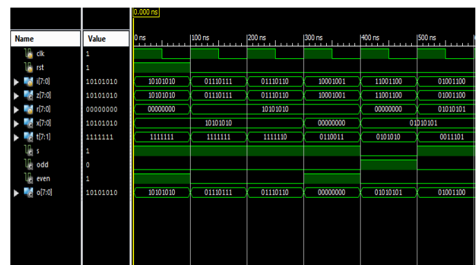
Fig.11. Scheme 3 Decoder
