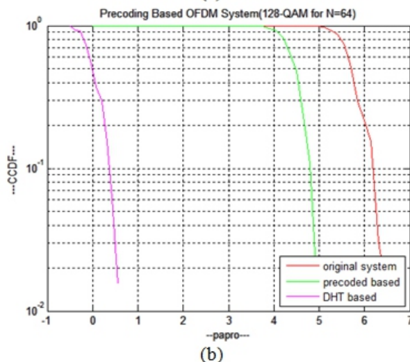
Fig. 3 (a) proposed PAPR reduction with 64-QAM for N=64 (b) 128-QAM for N=64
