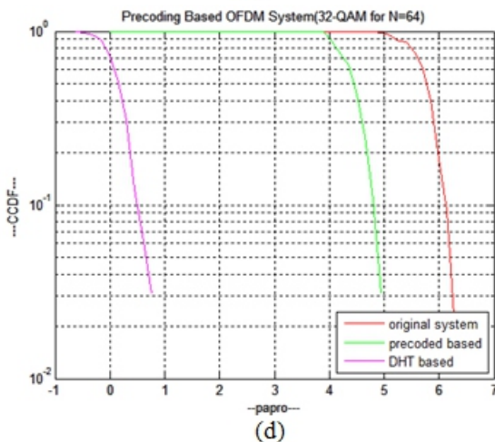
Fig. 2 (a) PAPR comparison for companding and exponential methods (b) BER performance (c) Proposed PAPR reduction for 16-QAM and N=64 (d) Proposed PAPR reduction for 32-QAM and N=64.
