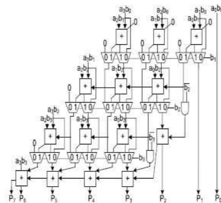
Fig. 3. 4 × 4 row-bypassing multiplier
