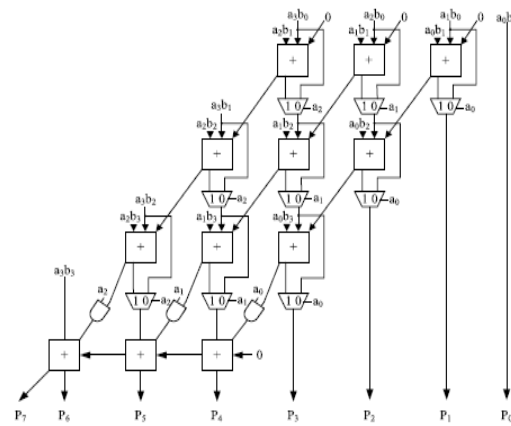
Fig. 2. 4 × 4 column-bypassing multiplier
