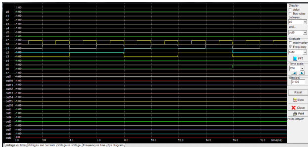
Fig 20: Simulation of Layout of 8x8 Vedic Multiplier
