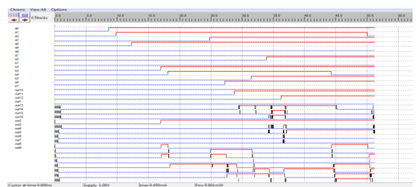
Fig 18: Timing Diagram of 8x8 Vedic Multiplier
