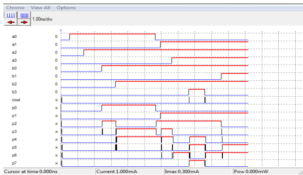
Fig 14: Timing Diagram of 4x4 Vedic Multiplier
