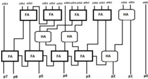
Fig. 8 4-bit multiplier design1
