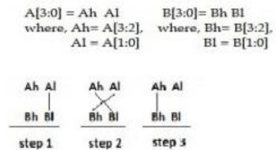
Fig. 2 Line diagram for binary multiplication using UT sutra
