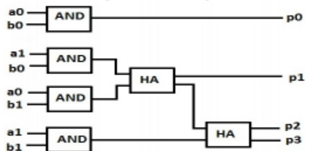
Fig. 7 UT based 2-bit Multiplier Architecture
