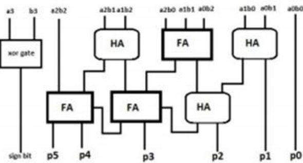
Fig. 10 4-bit signed multiplier
