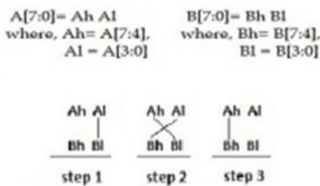
Fig. 11 8-bit multiplication using 2-bit UT multiplication analogy
