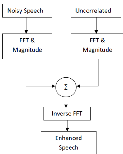
Fig.3: Spectral subtraction speech enhancement
