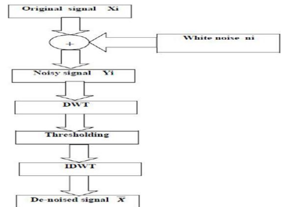
Fig.4: Denoised algorithm
