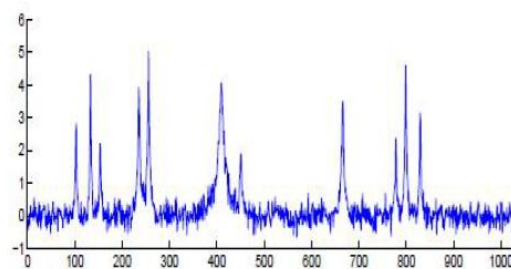
Fig.6: Noisy signal
