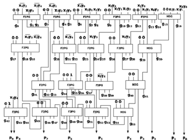
Fig 13. Circuit of 5x5 fault tolerant reversible signed multiplier.
