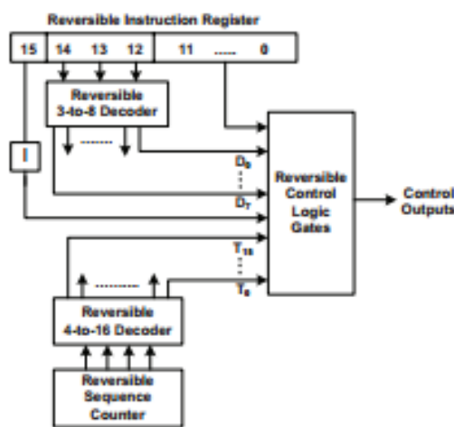
Fig. 8. Proposed Reversible Control Unit
