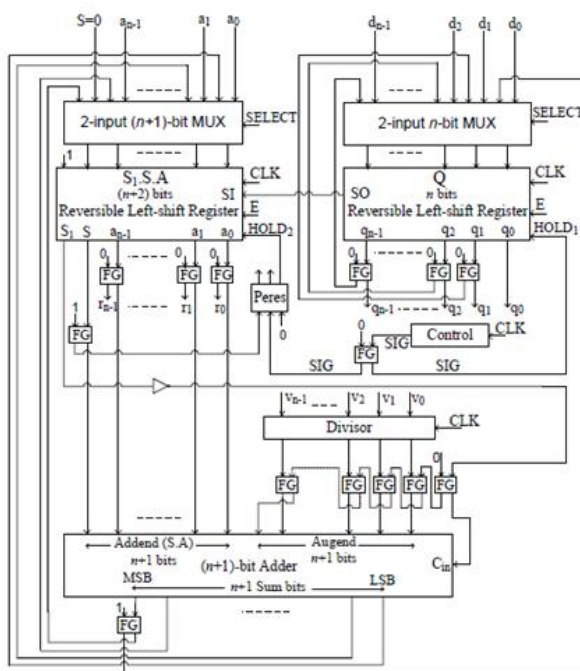
Figure 14. Proposed n-bit reversible division circuit
