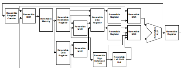
Fig: Data path Design of the Proposed Reversible Processor
