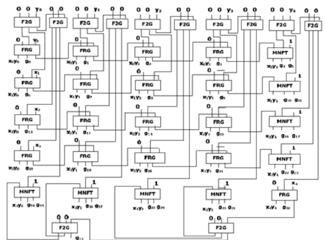
Fig 12.5. 5 fault tolerant reversible partial products generation circuit.
