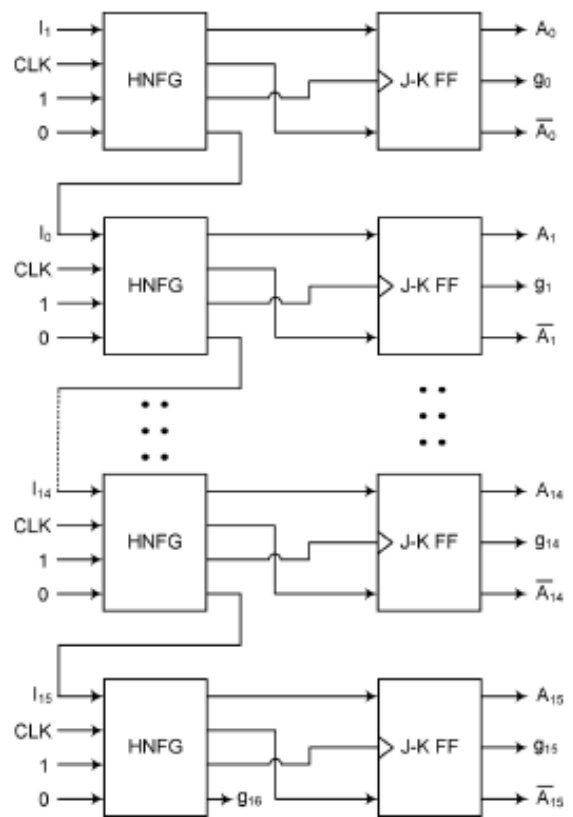
Fig. 4. Proposed designs of 16-bit reversible instruction register.
