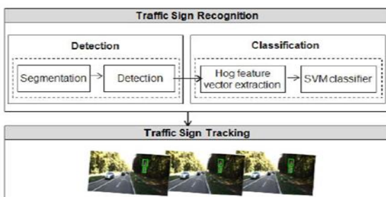
Figure1: The proposed traffic indication recognition and tracking process.
