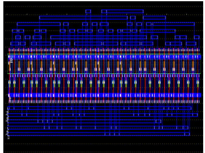
Fig 12: Layout of GDI 12T Full adder
