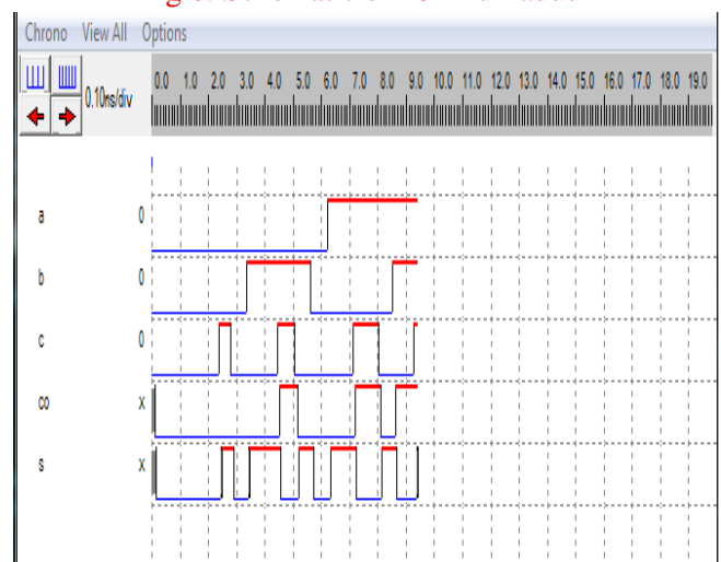
Fig 7: Timing Diagram of 28T Full adder
