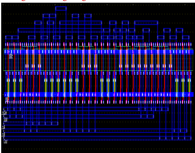
Fig 16: Layout of GDI 10T Full adder
