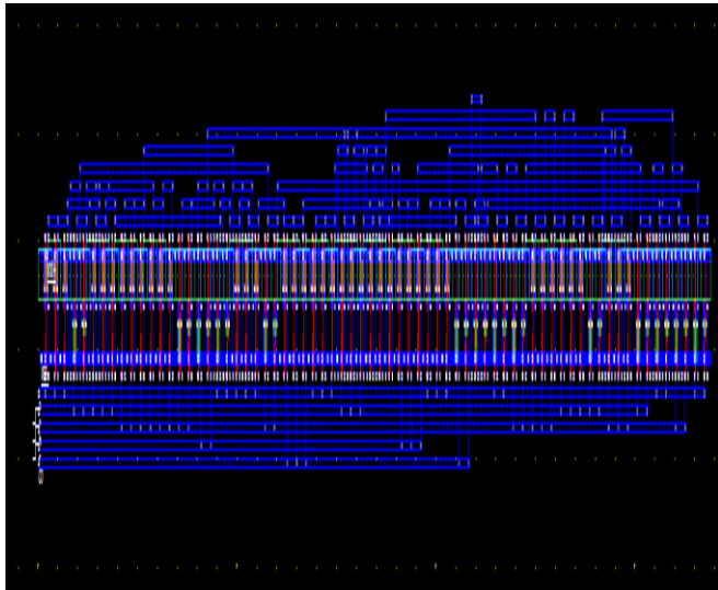
Fig 8: Layout of 28T Full adder
