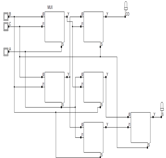
Fig.4 Block Diagram of Low Power Proposed Full Adder using 2T MUX
