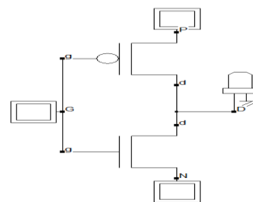
Fig 2 GDI basic cell consisting of pMOS and nMOS
