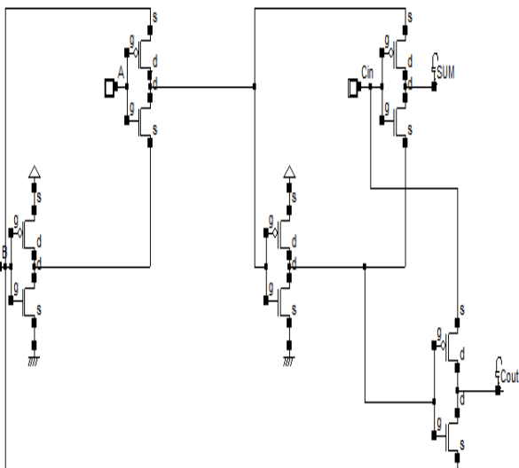
Fig. 5. GDI based 1-bit full adder cell
