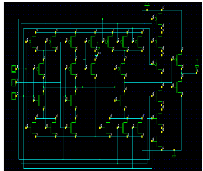
Fig 6: Schematic of 28T Full adder
