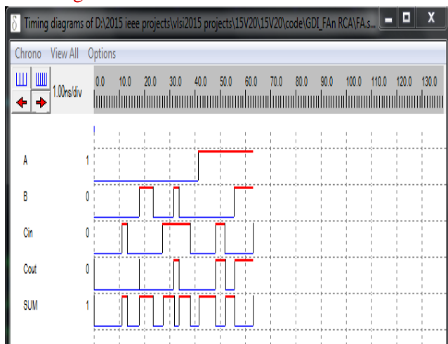
Fig 15: Timing Diagram of GDI 10T Full adder
