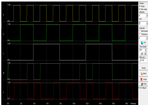
Fig 9: Simulation of Layout of 28T Full adder
