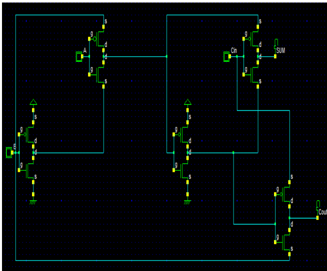
Fig 14: Schematic of GDI 10T Full adder
