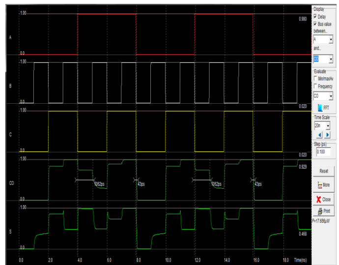
Fig 13: Simulation of Layout GDI 12T Full adder
