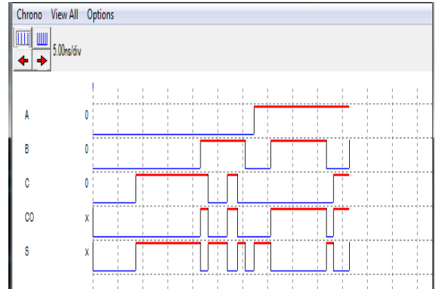
Fig 11: Timing Diagram of GDI 12T Full adder
