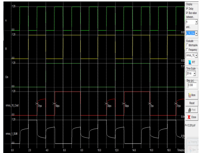
Fig 17: Simulation of Layout GDI 10T Full adder
