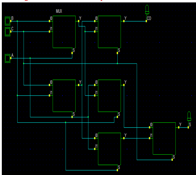
Fig 10: Schematic of GDI 12T Full adder
