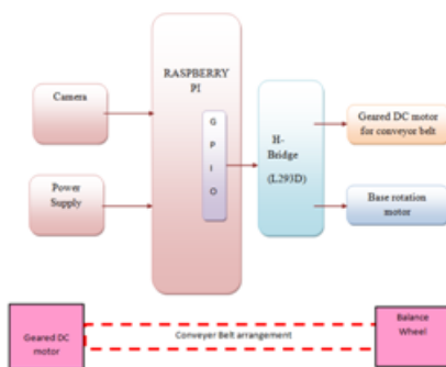
Fig. Block diag. of agriculture based object automatic sorting system
