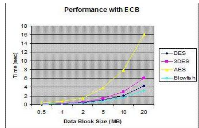
Fig 2. Encryption performance comparison with ECB
