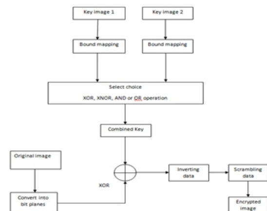
Fig.2 Proposed block diagram for Boundmap Crypt algorithm.
