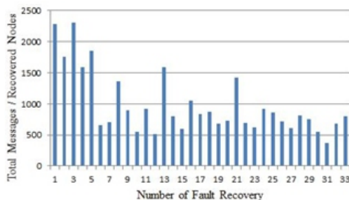
Fig. 17. Rate of total messages to recovery nodes.
