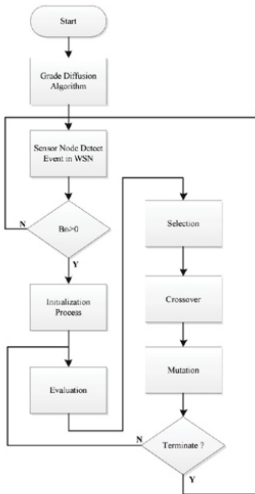
Fig. 3. Fault node recovery algorithm flow chart.
