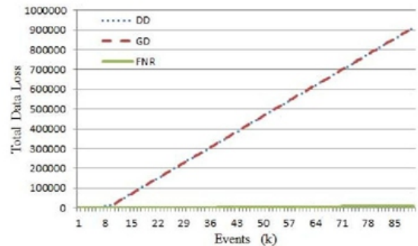
Fig. 9. Total data loss.
