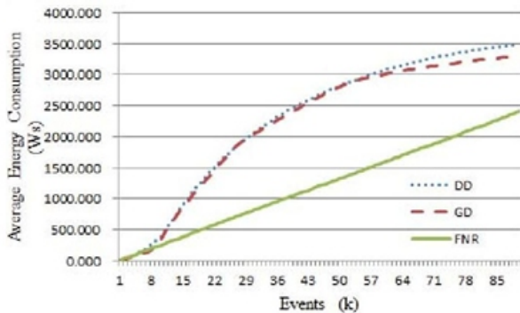
Fig. 10. Average energy consumption.
