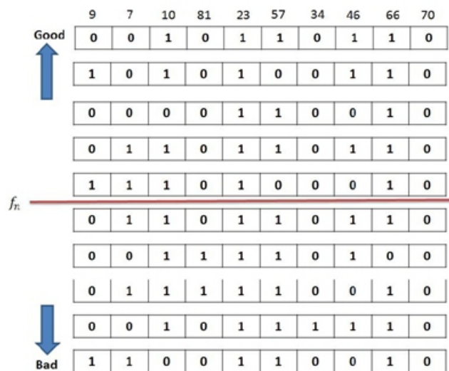
Fig. 5. Selection step.
